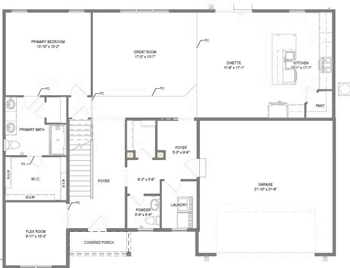
First Floor
