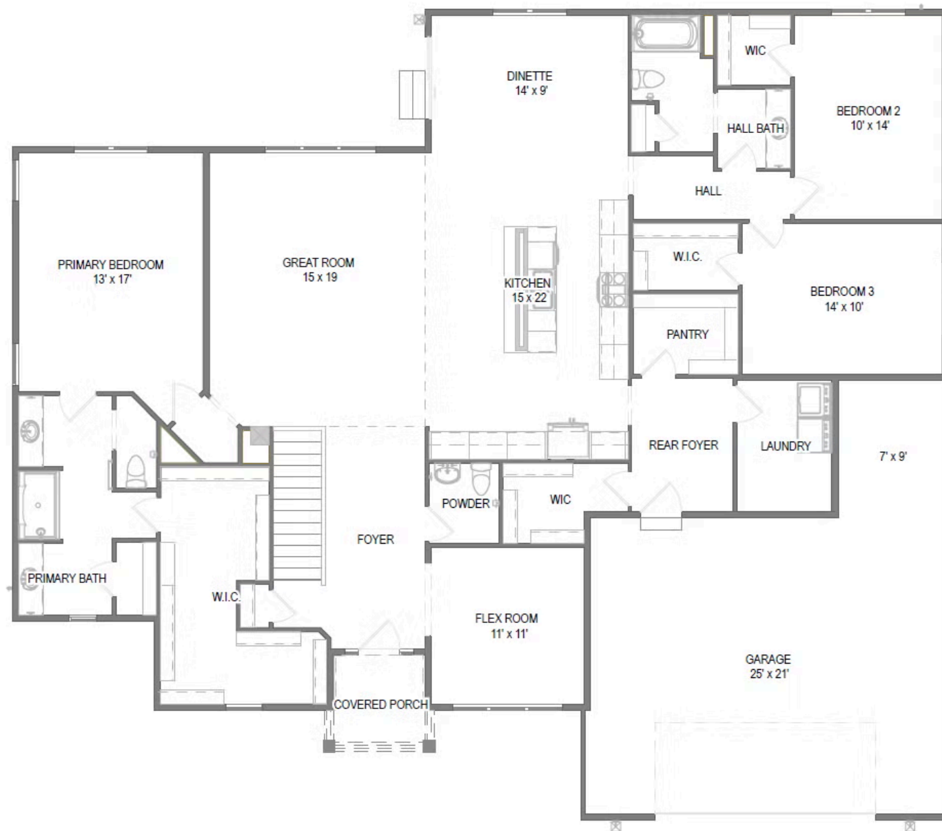
First Floor
