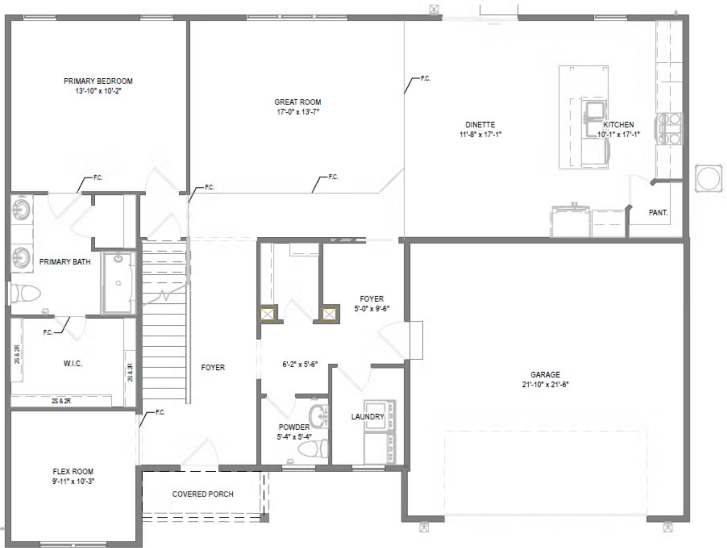
First Floor
