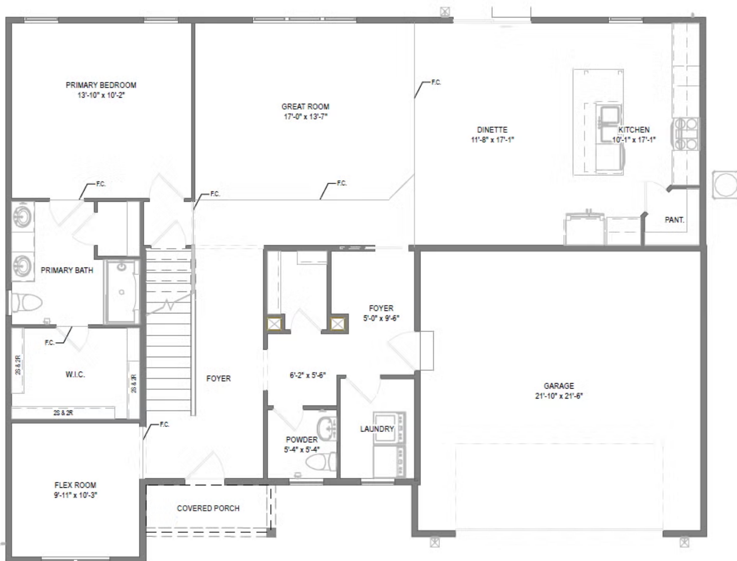
First Floor
