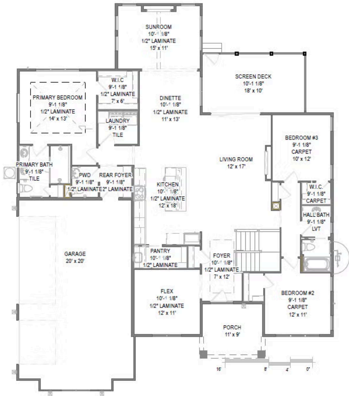
First Floor
