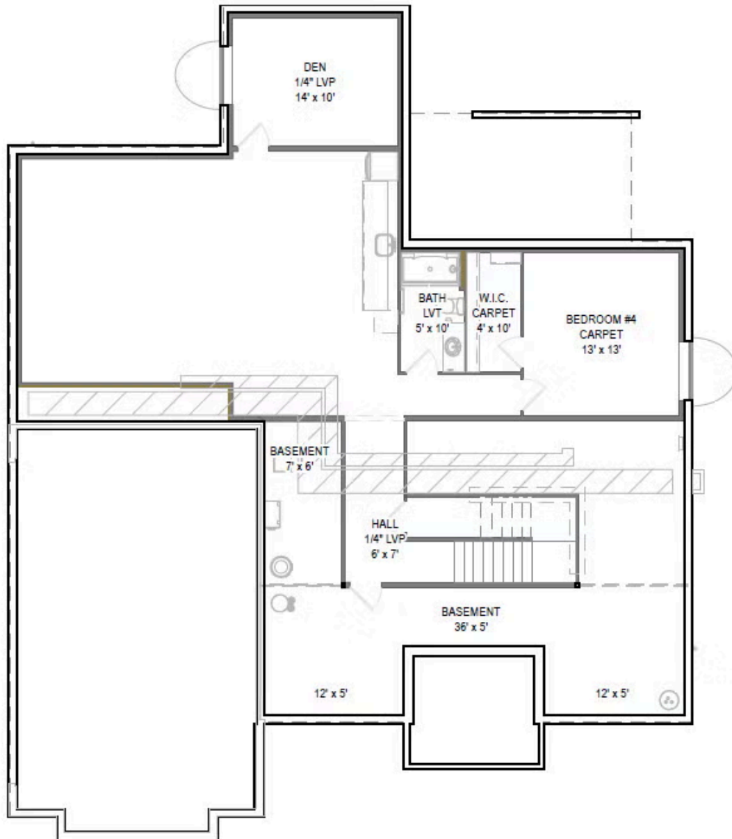
Basement
