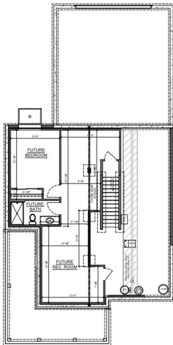
FOUNDATION FLOOR PLAN SCALE: 1/4"=1'-0"
