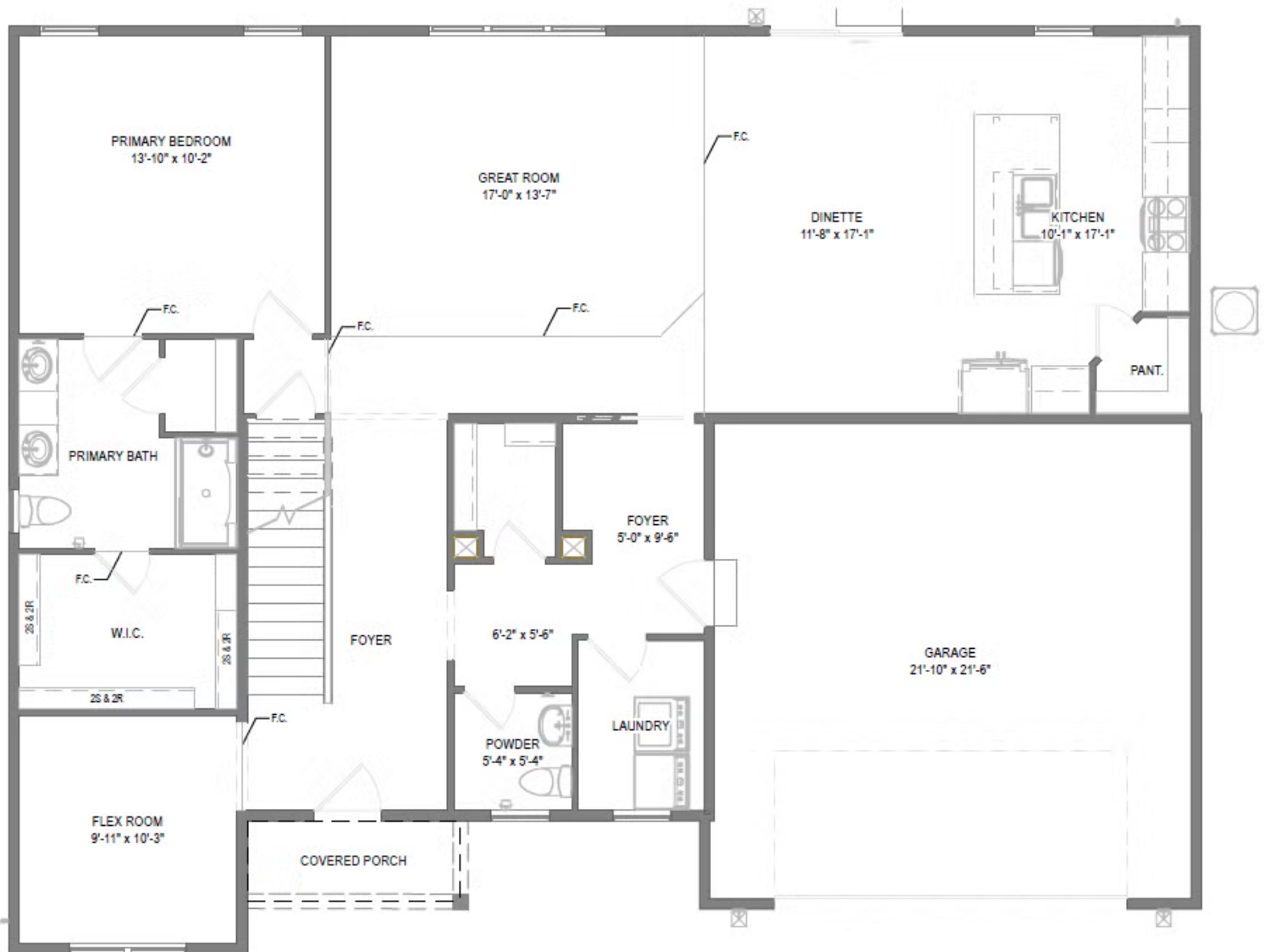
First Floor
