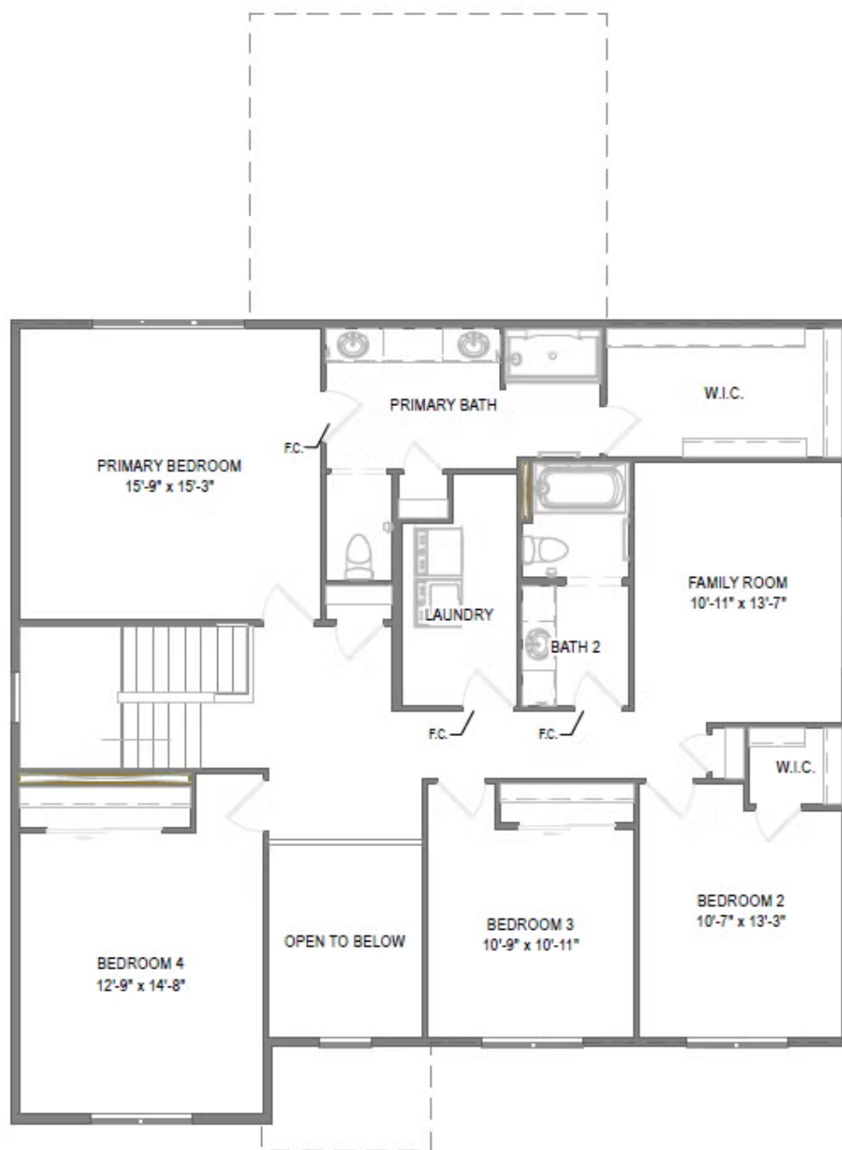
Second Floor
