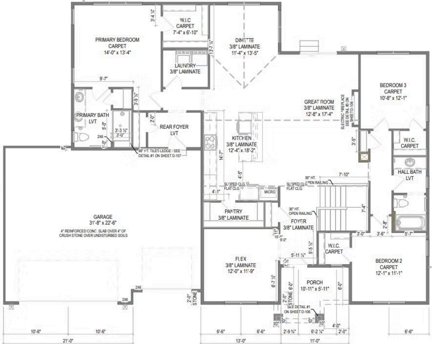
First Floor
