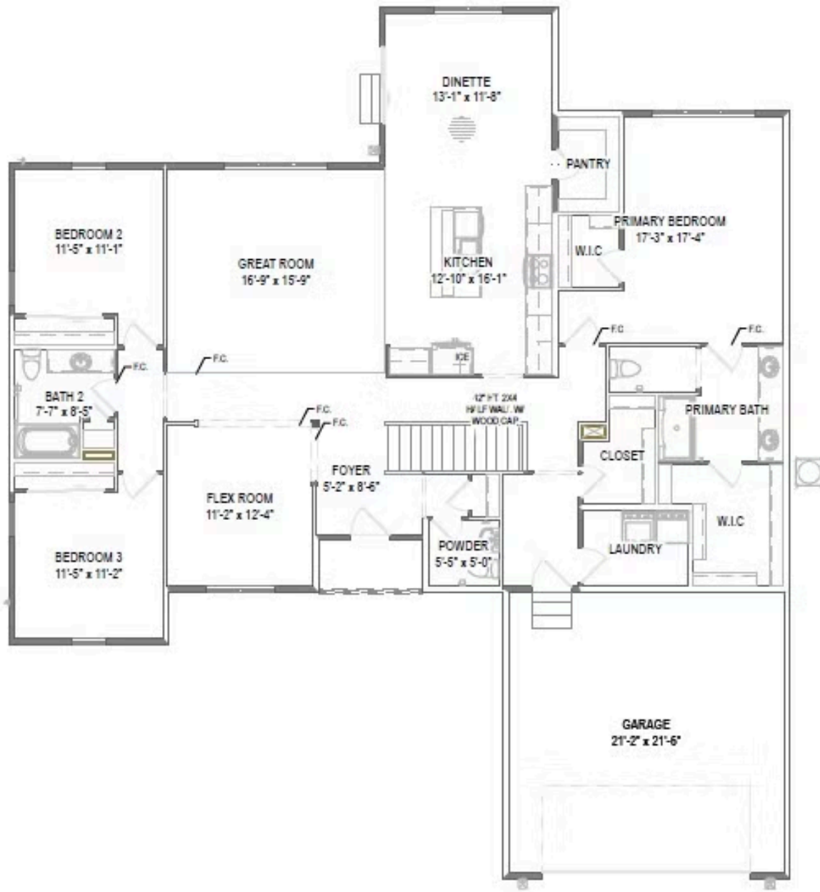
First Floor
