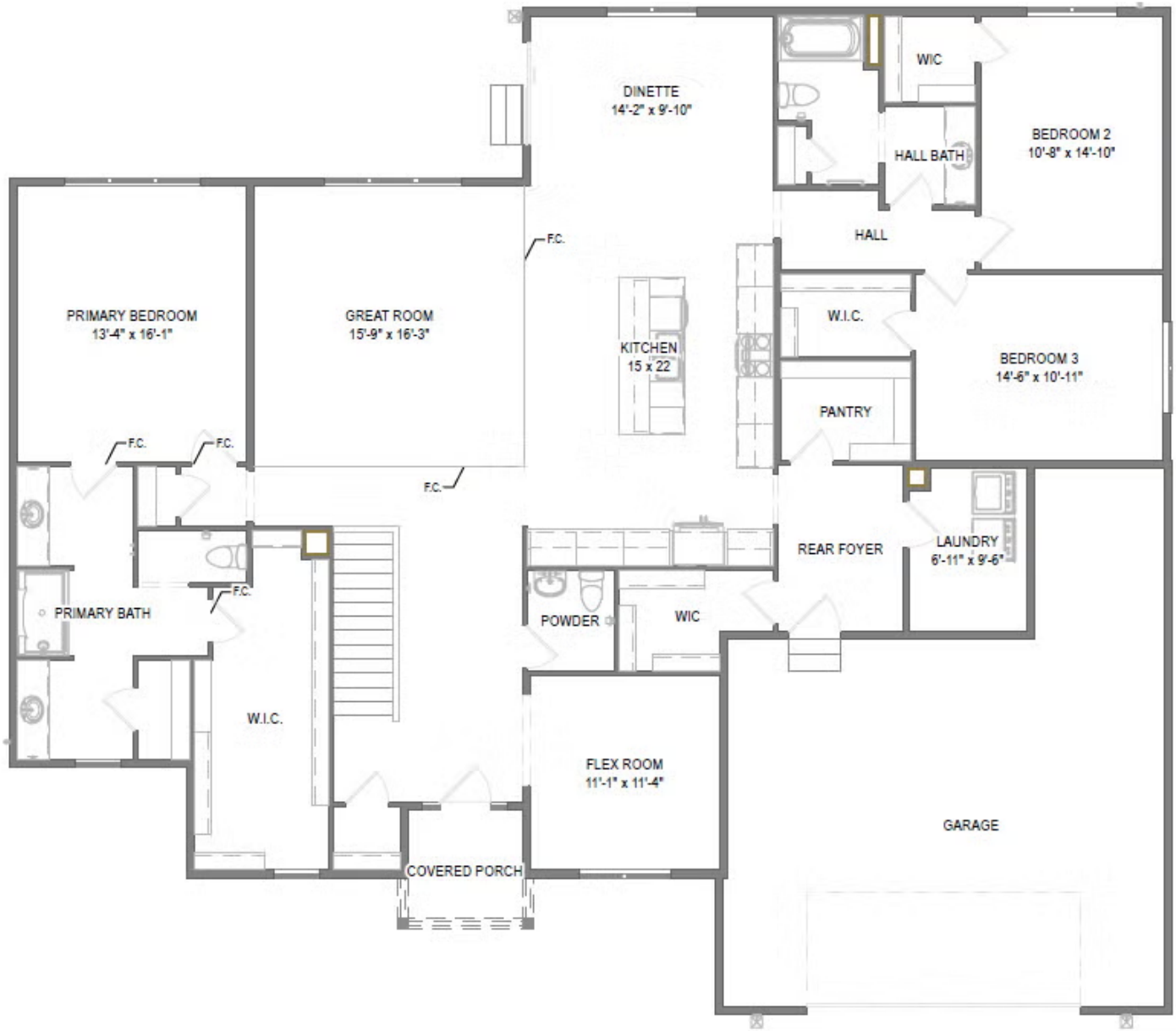
First Floor
